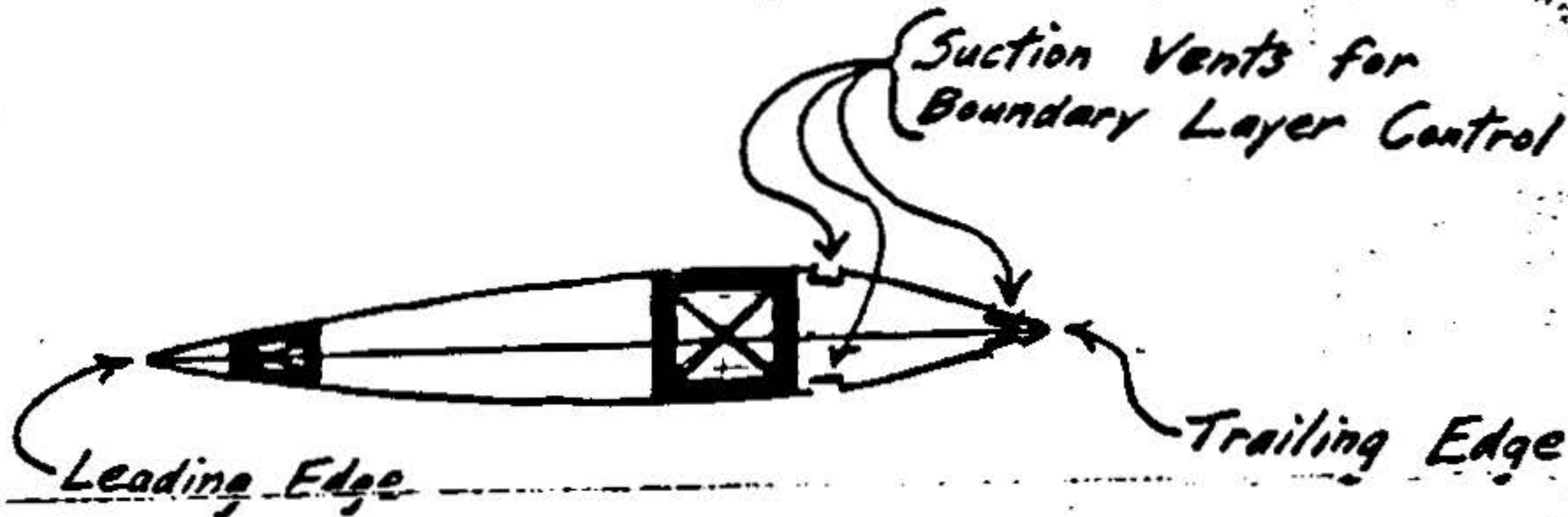
Airfoil Section (Becomes Relatively Thinner Near Wing Tips) Exhibit C
